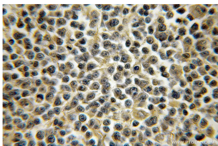
Immunohistochemical analysis of paraffin-embedded human lymphoma using 12396-1-AP (RGS13 antibody) at dilution of 1:50 (under 10x lens).
