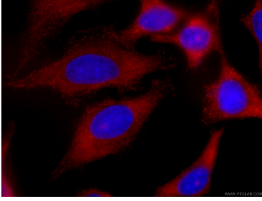
Immunofluorescent analysis of (-20°C Ethanol) fixed HeLa cells using CL594-66024 (EIF3D antibody) at dilution of 1:100.
