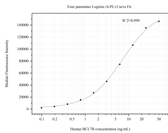
Cytometric bead array standard curve of MP50729-1, BCL7B Monoclonal Matched Antibody Pair, PBS Only. Capture antibody: 60517-1-PBS. Detection antibody: 60517-2-PBS. Standard:Ag22892. Range: 0.098-50 ng/mL
