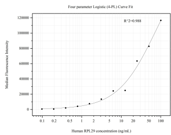
Cytometric bead array standard curve of MP50777-4, RPL29 Monoclonal Matched Antibody Pair, PBS Only. Capture antibody: 60552-3-PBS. Detection antibody: 60552-6-PBS. Standard:Ag8379. Range: 0.098-100 ng/mL
