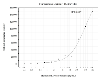
Cytometric bead array standard curve of MP50777-2, RPL29 Monoclonal Matched Antibody Pair, PBS Only. Capture antibody: 60552-3-PBS. Detection antibody: 60552-4-PBS. Standard:Ag8379. Range: 0.098-100 ng/mL
