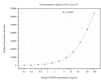
Cytometric bead array standard curve of MP51072-2, WDR78 Monoclonal Matched Antibody Pair, PBS Only. Capture antibody: 60742-3-PBS. Detection antibody: 60742-2-PBS. Standard:Ag27018. Range: 0.098-100 ng/mL
