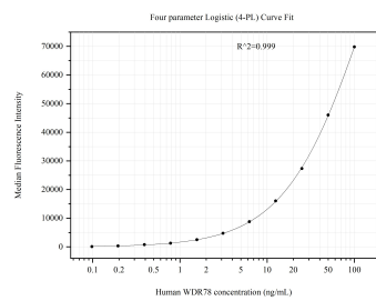
Cytometric bead array standard curve of MP51072-1, WDR78 Monoclonal Matched Antibody Pair, PBS Only. Capture antibody: 60742-1-PBS. Detection antibody: 60742-2-PBS. Standard:Ag27018. Range: 0.098-100 ng/mL
