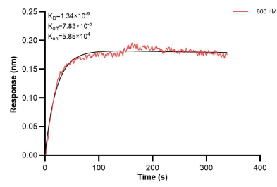
Biological layer interferometry (BLI) kinetic assays of 61074-2-Ig against Human HMGN2 were performed. The affinity constant is 1.34 nM.
