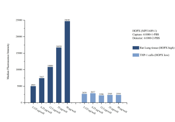
Cytometric bead array sample test of MP51689-1, HOPX Monoclonal Matched Antibody Pair, PBS Only. Capture antibody: 61080-1-PBS. Detection antibody: 61080-2-PBS.
