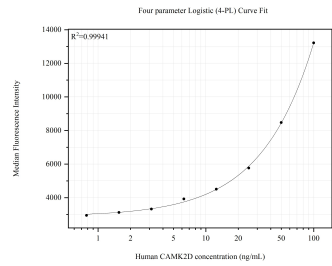
Cytometric bead array standard curve of MP51748-1, CAMK2D Monoclonal Matched Antibody Pair, PBS Only. Capture antibody: 61090-1-PBS. Detection antibody: 61090-2-PBS. Standard:Ag7323. Range: 0.781-100 ng/mL.
