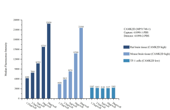
Cytometric bead array sample test of MP51748-1, CAMK2D Monoclonal Matched Antibody Pair, PBS Only. Capture antibody: 61090-1-PBS. Detection antibody: 61090-2-PBS.
