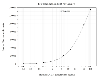
Cytometric bead array standard curve of MP50968-2, NOTUM Monoclonal Matched Antibody Pair, PBS Only. Capture antibody: 66956-2-PBS. Detection antibody: 66956-4-PBS. Standard:Ag6338. Range: 0.098-100 ng/mL
