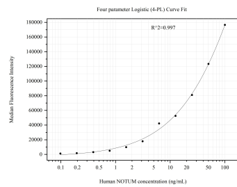
Cytometric bead array standard curve of MP50968-3, NOTUM Monoclonal Matched Antibody Pair, PBS Only. Capture antibody: 66956-2-PBS. Detection antibody: 66956-1-PBS. Standard:Ag6338. Range: 0.098-100 ng/mL
