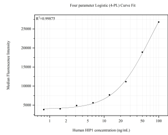
Cytometric bead array standard curve of MP51715-1, HIP1 Monoclonal Matched Antibody Pair, PBS Only. Capture antibody: 67163-2-PBS. Detection antibody: 67163-3-PBS. Standard:Ag17982. Range: 0.781-100 ng/mL.
