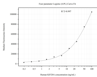
Cytometric bead array standard curve of MP51304-2, KIF20A Monoclonal Matched Antibody Pair, PBS Only. Capture antibody: 67190-4-PBS. Detection antibody: 67190-2-PBS. Standard:Ag8916. Range: 0.195-100 ng/mL
