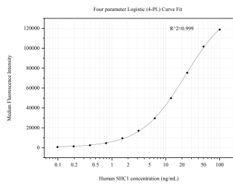
Cytometric bead array standard curve of MP50763-1, SHC1 Monoclonal Matched Antibody Pair, PBS Only. Capture antibody: 67194-2-PBS. Detection antibody: 67194-3-PBS. Standard:Ag25173. Range: 0.098-100 ng/mL
