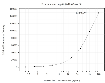
Cytometric bead array standard curve of MP50763-2, SHC1 Monoclonal Matched Antibody Pair, PBS Only. Capture antibody: 67194-3-PBS. Detection antibody: 67194-4-PBS. Standard:Ag25173. Range: 0.391-100 ng/mL
