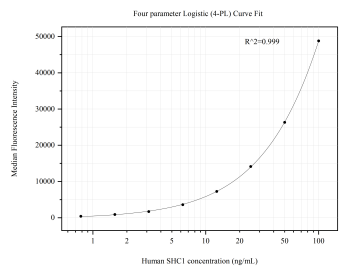
Cytometric bead array standard curve of MP50763-4, SHC1 Monoclonal Matched Antibody Pair, PBS Only. Capture antibody: 67194-5-PBS. Detection antibody: 67194-3-PBS. Standard:Ag25173. Range: 0.781-100 ng/mL
