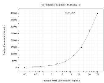
Cytometric bead array standard curve of MP51017-2, ERO1L Monoclonal Matched Antibody Pair, PBS Only. Capture antibody: 67416-2-PBS. Detection antibody: 67416-4-PBS. Standard:Ag29910. Range: 0.195-100 ng/mL
