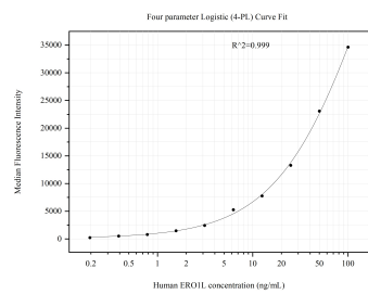
Cytometric bead array standard curve of MP51017-1, ERO1L Monoclonal Matched Antibody Pair, PBS Only. Capture antibody: 67416-2-PBS. Detection antibody: 67416-3-PBS. Standard:Ag29910. Range: 0.195-100 ng/mL
