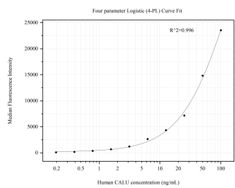
Cytometric bead array standard curve of MP50698-2, CALU Monoclonal Matched Antibody Pair, PBS Only. Capture antibody: 67585-2-PBS. Detection antibody: 67585-1-PBS. Standard:Ag12073. Range: 0.195-100 ng/mL
