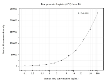
Cytometric bead array standard curve of MP50572-3, Prx5 Monoclonal Matched Antibody Pair, PBS Only. Capture antibody: 67599-4-PBS. Detection antibody: 67599-5-PBS. Standard:Ag12262. Range: 0.098-100 ng/mL
