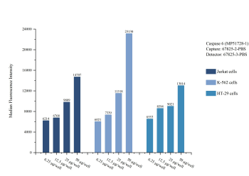
Cytometric bead array sample test of MP51728-1, Caspase 6 Monoclonal Matched Antibody Pair, PBS Only. Capture antibody: 67825-2-PBS. Detection antibody: 67825-3-PBS.
