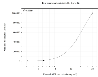
Cytometric bead array standard curve of MP51721-1, PAIP1 Monoclonal Matched Antibody Pair, PBS Only. Capture antibody: 68042-2-PBS. Detection antibody: 68042-3-PBS. Standard: Ag16773. Range: 3.13-50 ng/mL
