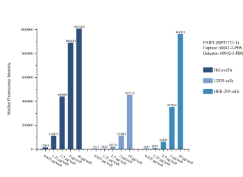
Cytometric bead array sample test of MP51721-1, PAIP1 Monoclonal Matched Antibody Pair, PBS Only. Capture antibody: 68042-2-PBS. Detection antibody: 68042-3-PBS.
