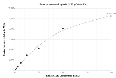
Cytometric bead array standard curve of MP01853-1, STAT2 Recombinant Matched Antibody Pair, PBS Only. Capture antibody: 80061-3-PBS. Detection antibody: 80061-4-PBS. Standard: Ag10168. Range: 1.563-200 ng/mL.
