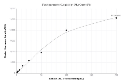
Cytometric bead array standard curve of MP01853-2, STAT2 Recombinant Matched Antibody Pair, PBS Only. Capture antibody: 80061-2-PBS. Detection antibody: 80061-4-PBS. Standard: Ag10168. Range: 1.563-200 ng/mL.
