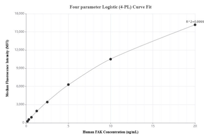
Cytometric bead array standard curve of MP02124-2, FAK Recombinant Matched Antibody Pair, PBS Only. Capture antibody: 81334-4-PBS. Detection antibody: 81334-3-PBS. Standard: Ag3331. Range: 0.156-20 ng/mL
