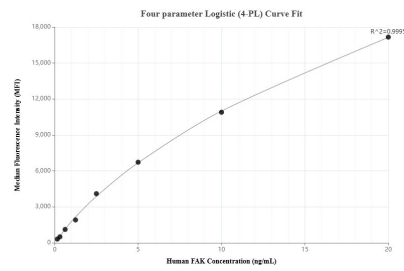
Cytometric bead array standard curve of MP02124-1, FAK Recombinant Matched Antibody Pair, PBS Only. Capture antibody: 81334-4-PBS. Detection antibody: 81334-2-PBS. Standard: Ag3331. Range: 0.156-20 ng/mL
