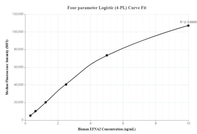
Cytometric bead array standard curve ofMP00081-1, EFNA2 Recombinant Matched Antibody Pair, PBS Only. Capture antibody: 82951-5-PBS. Detection antibody: 82951-4-PBS. Standard: SY00429. Range: 0.313-10 ng/mL
