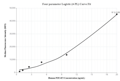
Cytometric bead array standard curve ofMP00087-3, POU4F3 Recombinant Matched Antibody Pair, PBS Only. Capture antibody: 82980-4-PBS. Detection antibody: 82980-3-PBS. Standard: Ag16004. Range: 0.625-20 ng/mL.
