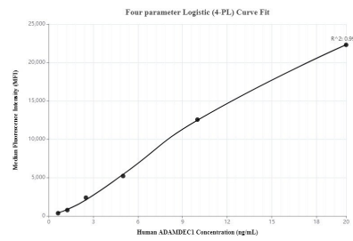
Cytometric bead array standard curve of MP00007-3, ADAMDEC1 Recombinant Matched Antibody Pair, PBS Only. Capture antibody: 82985-2-PBS. Detection antibody: 82985-5-PBS. Standard:Ag12265. Range: 0.625-20 ng/mL
