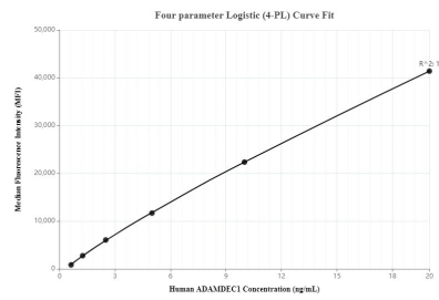
Cytometric bead array standard curve of MP00007-1, ADAMDEC1 Recombinant Matched Antibody Pair, PBS Only. Capture antibody: 82985-5-PBS. Detection antibody: 82985-4-PBS. Standard:Ag12265. Range: 0.625-20 ng/mL
