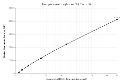
Cytometric bead array standard curve of MP00007-2, ADAMDEC1 Recombinant Matched Antibody Pair, PBS Only. Capture antibody: 82985-5-PBS. Detection antibody: 82985-3-PBS. Standard:Ag12265. Range: 0.625-20 ng/mL
