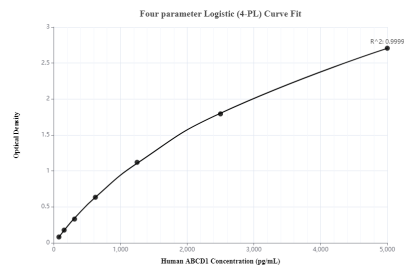
Sandwich ELISA standard curve ofMP00070-2, ABCD1 Recombinant Matched Antibody Pair, PBS Only. Capture antibody: 83038-2-PBS. Detection antibody: 83038-3-PBS. Standard: Ag0453. Range: 78-5000 pg/mL
