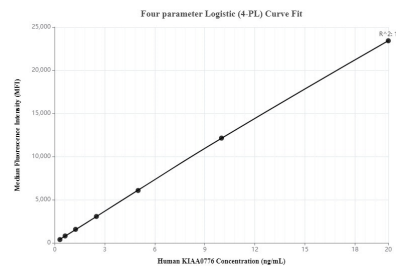
Cytometric bead array standard curve ofMP00135-2, KIAA0776 Recombinant Matched Antibody Pair, PBS Only. Capture antibody: 83047-1-PBS. Detection antibody: 83047-4-PBS. Standard: Ag23362. Range: 0.313-20 ng/mL
