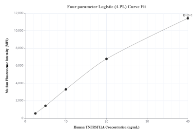
Cytometric bead array standard curve of MP00249-1, TNFRSF 11A Recombinant Matched Antibody Pair, PBS Only. Capture antibody: 83253-2-PBS. Detection antibody: 83253-1-PBS. Standard: Ag29425. Range: 2.5-40 ng/mL.
