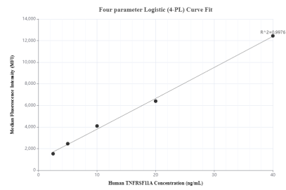
Cytometric bead array standard curve of MP00249-2, TNFRSF 11A Recombinant Matched Antibody Pair, PBS Only. Capture antibody: 83253-2-PBS. Detection antibody: 83253-3-PBS. Standard: Ag29425. Range: 2.5-40 ng/mL.
