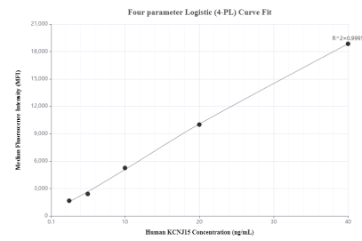
Cytometric bead array standard curve ofMP00164-3, KCNJ15 Recombinant Matched Antibody Pair, PBS Only. Capture antibody: 83257-1-PBS. Detection antibody: 83257-3-PBS. Standard: Ag34655. Range: 2.5-40 ng/mL
