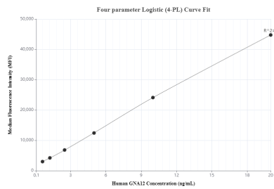
Cytometric bead array standard curve ofMP00276-2, GNA12 Recombinant Matched Antibody Pair, PBS Only. Capture antibody: 83263-1-PBS. Detection antibody: 83263-2-PBS. Standard: Ag35068. Range: 0.625-20 ng/mL
