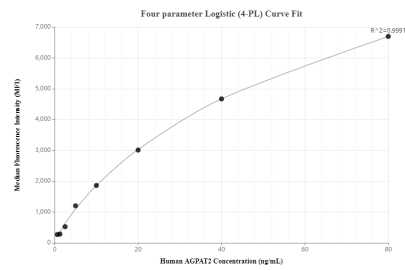
Cytometric bead array standard curve of MP00360-3, AGPAT2 Recombinant Matched Antibody Pair, PBS Only. Capture antibody: 83349-4-PBS. Detection antibody: 83349-1-PBS. Standard: Ag34761. Range: 0.625-80 ng/mL.
