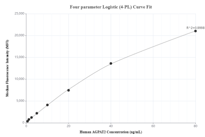
Cytometric bead array standard curve of MP00360-1, AGPAT2 Recombinant Matched Antibody Pair, PBS Only. Capture antibody: 83349-2-PBS. Detection antibody: 83349-4-PBS. Standard: Ag34761. Range: 0.625-80 ng/mL.
