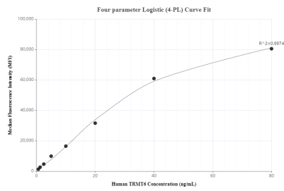
Cytometric bead array standard curve of MP00816-1, TRMT6 Recombinant Matched Antibody Pair, PBS Only. Capture antibody: 83843-4-PBS. Detection antibody: 83843-2-PBS. Standard: Ag10176. Range: 0.625-80 ng/mL
