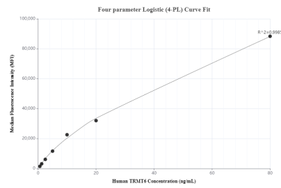
Cytometric bead array standard curve of MP00816-2, TRMT6 Recombinant Matched Antibody Pair, PBS Only. Capture antibody: 83843-1-PBS. Detection antibody: 83843-4-PBS. Standard: Ag10176. Range: 0.625-80 ng/mL
