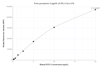
Cytometric bead array standard curve of MP00840-1, Perilipin 1 Recombinant Matched Antibody Pair, PBS Only. Capture antibody: 83905-1-PBS. Detection antibody: 83905-2-PBS. Standard: Ag26426. Range: 0.156-20 ng/mL.
