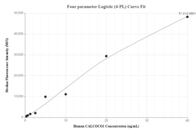
Cytometric bead array standard curve of MP00945-1, CALCOCO1 Recombinant Matched Antibody Pair, PBS Only. Capture antibody: 84009-2-PBS. Detection antibody: 84009-3-PBS. Standard: Ag13876. Range: 0.313-40 ng/mL.
