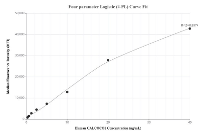
Cytometric bead array standard curve of MP00945-2, CALCOCO1 Recombinant Matched Antibody Pair, PBS Only. Capture antibody: 84009-1-PBS. Detection antibody: 84009-3-PBS. Standard: Ag13876. Range: 0.313-40 ng/mL.
