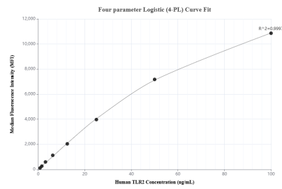
Cytometric bead array standard curve of MP01332-3, TLR2 Recombinant Matched Antibody Pair, PBS Only. Capture antibody: 84462-2-PBS. Detection antibody: 84462-3-PBS. Standard: RP00009. Range: 0.781-100 ng/mL.
