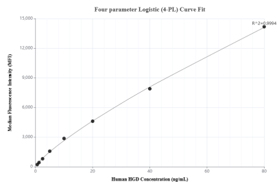
Cytometric bead array standard curve of MP01681-2, HGD Recombinant Matched Antibody Pair, PBS Only. Capture antibody: 84931-3-PBS. Detection antibody: 84931-1-PBS. Standard: Ag9544. Range: 0.625-80 ng/mL
