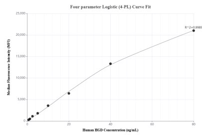
Cytometric bead array standard curve of MP01681-1, HGD Recombinant Matched Antibody Pair, PBS Only. Capture antibody: 84931-3-PBS. Detection antibody: 84931-2-PBS. Standard: Ag9544. Range: 0.625-80 ng/mL
