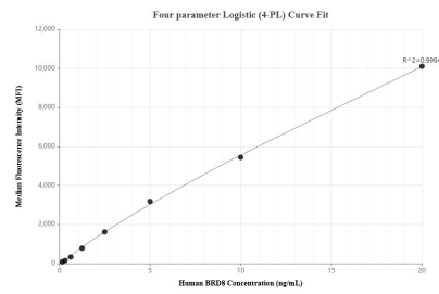
Cytometric bead array standard curve of MP01679-2, BRD8 Recombinant Matched Antibody Pair, PBS Only. Capture antibody: 84965-2-PBS. Detection antibody: 84965-3-PBS. Standard: Ag0790. Range: 0.156-20 ng/mL
