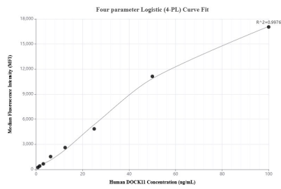
Cytometric bead array standard curve of MP01759-1, DOCK11 Recombinant Matched Antibody Pair, PBS Only. Capture antibody: 85022-2-PBS. Detection antibody: 85022-1-PBS. Standard: Ag35831. Range: 0.781-100 ng/mL
