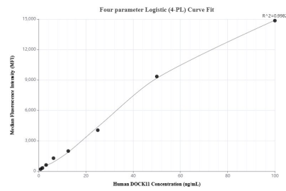
Cytometric bead array standard curve of MP01759-2, DOCK11 Recombinant Matched Antibody Pair, PBS Only. Capture antibody: 85022-3-PBS. Detection antibody: 85022-1-PBS. Standard: Ag35831. Range: 0.781-100 ng/mL
