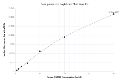
Cytometric bead array standard curve of MP01819-1, RNF128 Recombinant Matched Antibody Pair, PBS Only. Capture antibody: 85137-3-PBS. Detection antibody: 85137-1-PBS. Standard: Ag22834. Range: 0.625-40 ng/mL
