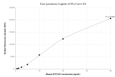
Cytometric bead array standard curve of MP01819-2, RNF128 Recombinant Matched Antibody Pair, PBS Only. Capture antibody: 85137-3-PBS. Detection antibody: 85137-2-PBS. Standard: Ag22834. Range: 0.625-40 ng/mL
