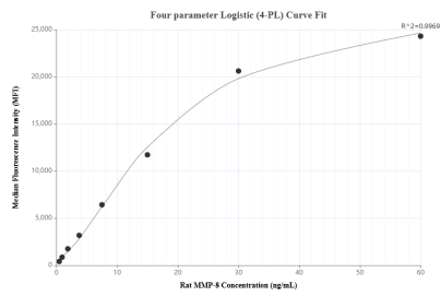
Cytometric bead array standard curve of MP01911-2, RAT MMP-8 Recombinant Matched Antibody Pair, PBS Only. Capture antibody: 85211-1-PBS. Detection antibody: 85211-3-PBS. Standard:Eg3278. Range: 0.469-60 ng/mL.
