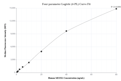
Cytometric bead array standard curve of MP02006-1, MEOX1 Recombinant Matched Antibody Pair, PBS Only. Capture antibody: 85618-1-PBS. Detection antibody: 85618-3-PBS. Standard: Ag12910. Range: 0.625-80 ng/mL
