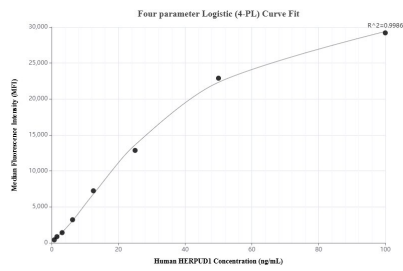
Cytometric bead array standard curve of MP02032-1, HERPUD1 Recombinant Matched Antibody Pair, PBS Only. Capture antibody: 85627-4-PBS. Detection antibody: 85627-3-PBS. Standard: Ag34891. Range: 0.781-100 ng/mL
