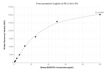
Cytometric bead array standard curve of MP02032-2, HERPUD1 Recombinant Matched Antibody Pair, PBS Only. Capture antibody: 85627-3-PBS. Detection antibody: 85627-2-PBS. Standard: Ag34891. Range: 0.781-100 ng/mL
