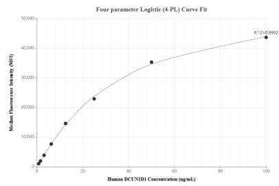
Cytometric bead array standard curve of MP02158-1, DCUN1D1 Recombinant Matched Antibody Pair, PBS Only. Capture antibody: 85849-3-PBS. Detection antibody: 85849-1-PBS. Standard: Ag1440. Range: 0.781-100 ng/mL
