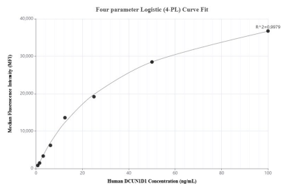
Cytometric bead array standard curve of MP02158-2, DCUN1D1 Recombinant Matched Antibody Pair, PBS Only. Capture antibody: 85849-3-PBS. Detection antibody: 85849-2-PBS. Standard: Ag1440. Range: 0.781-100 ng/mL
