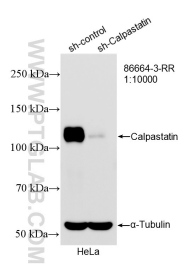
WB result of Calpastatin antibody (86664-3-RR; 1:10000; incubated at room temperature for 1.5 hours) with sh-Control and sh-Calpastatin transfected HeLa cells.
