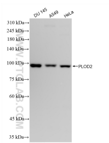
Various lysates were subjected to SDS PAGE followed by western blot with 88222-2-RR (PLOD2 antibody) at dilution of 1:10000 incubated at room temperature for 1.5 hours.
