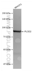
NIH/3T3 cells were subjected to SDS PAGE followed by western blot with 88222-2-RR (PLOD2 antibody) at dilution of 1:5000 incubated at room temperature for 1.5 hours.
