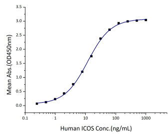
Immobilized Human ICOSLG (Myc tag, His tag) at 0.5 µg/mL (100 µL/well) can bind Human ICOS (hFc tag, Myc tag, His tag) with a linear range of 6-24 ng/mL
