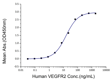
Immobilized Human VEGF165 (His tag) at 0.1 µg/mL (100 µL/well) can bind Human VEGFR2 (hFc tag) with a linear range of 7-30 ng/mL
