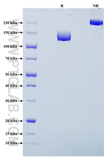
Purity of Recombinant Human VEGFR2 was determined by SDS-PAGE. The protein was resolved in an SDS-PAGE in reducing (R) and non-reducing (NR) conditions and stained using Coomassie blue.
