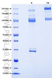
Purity of Recombinant Mouse MST1R was determined by SDS-PAGE. The protein was resolved in an SDS-PAGE in reducing (R) and non-reducing (NR) conditions and stained using Coomassie blue.
