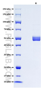
Purity of Recombinant Mouse IL-28B was determined by SDS-PAGE. The protein was resolved in an SDS-PAGE in reducing (R) conditions and stained using Coomassie blue.
