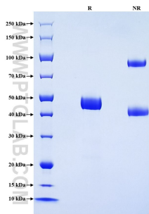
Purity of Recombinant Rat CD90 was determined by SDS-PAGE. The protein was resolved in an SDS-PAGE in reducing (R) and non-reducing (NR) conditions and stained using Coomassie blue.
