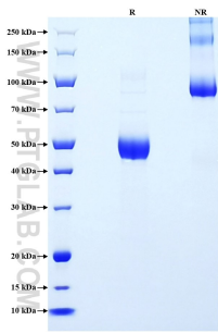
Purity of Recombinant Mouse IL-7 was determined by SDS-PAGE. The protein was resolved in an SDS-PAGE in reducing (R) and non-reducing (NR) conditions and stained using Coomassie blue.
