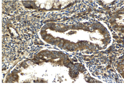
Immunohistochemical analysis of paraffin-embedded human cervical cancer tissue slide using KHC2059 (IFIT3 IHC Kit).
