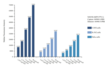
Cytometric bead array sample test of MP51579-1, NDC80 Monoclonal Matched Antibody Pair, PBS Only. Capture antibody: 66960-2-PBS. Detection antibody: 66960-3-PBS.
