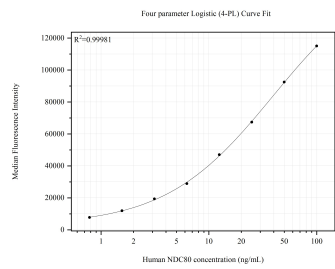
Cytometric bead array standard curve of MP51579-1, NDC80 Monoclonal Matched Antibody Pair, PBS Only. Capture antibody: 66960-2-PBS. Detection antibody: 66960-3-PBS. Standard:Ag8065. Range: 0.781-100 ng/mL.
